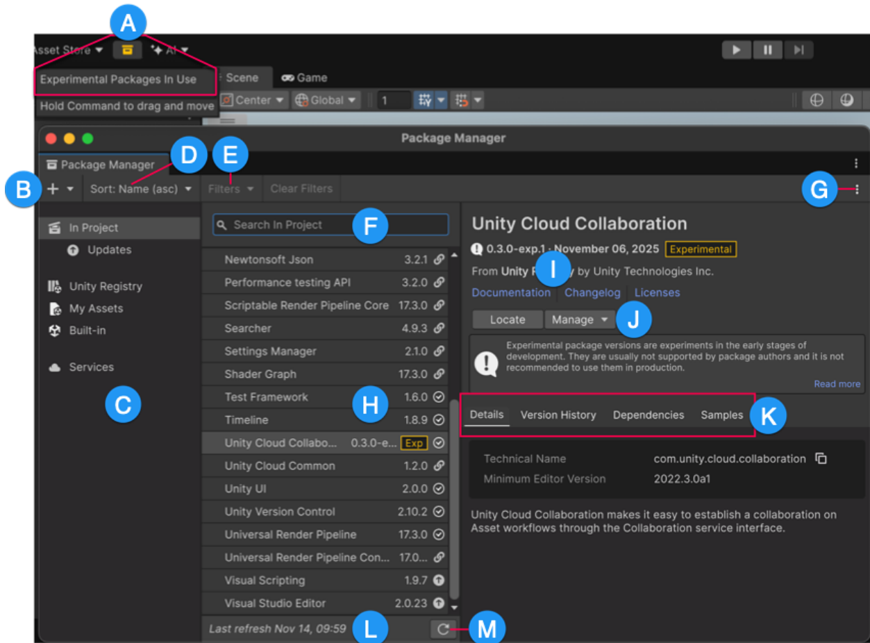
Fig. 5.1: Package Manager window
